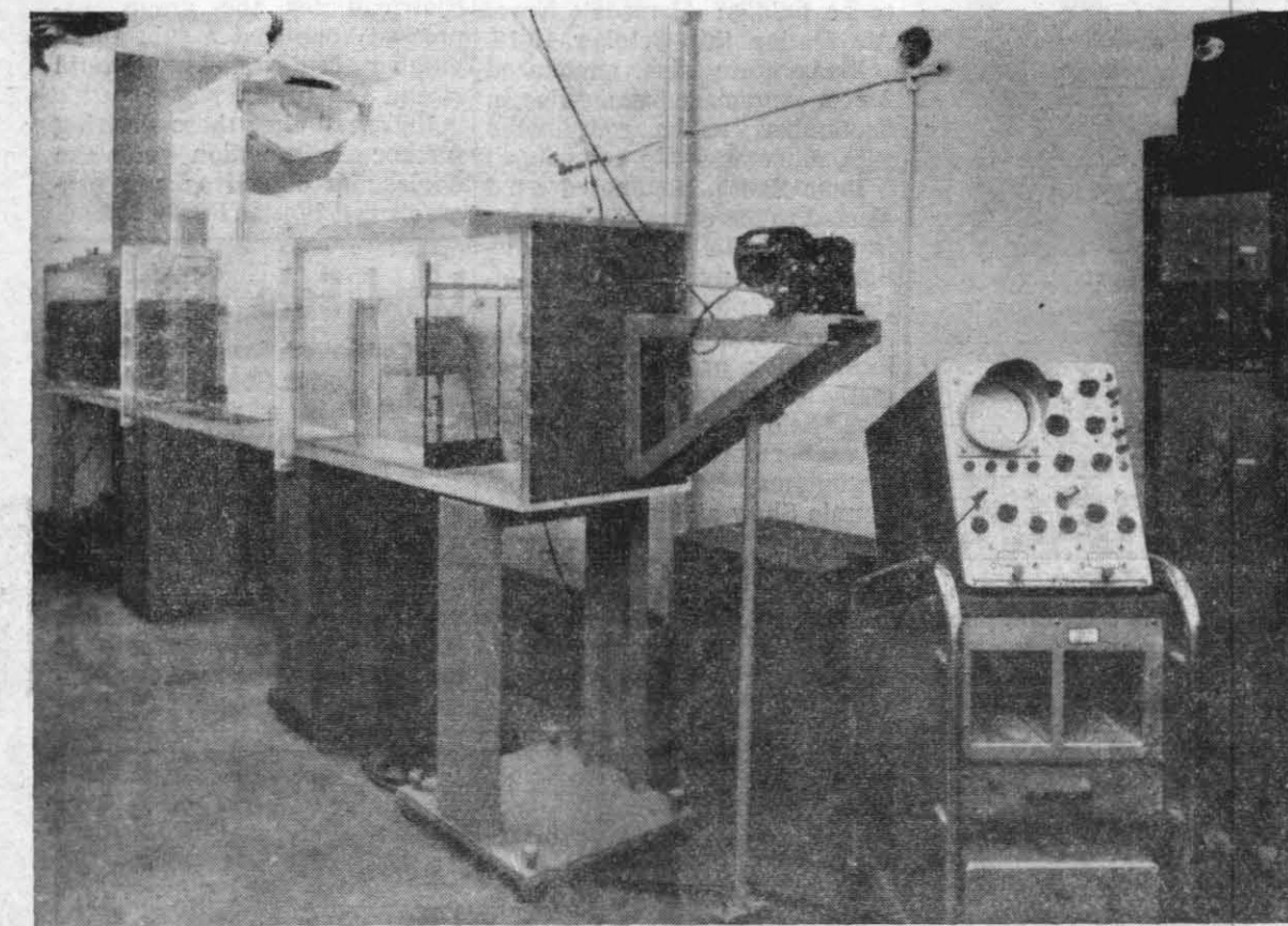
UNIQUE FACILITY, the Variable-Atmosphere Wave Tank, used by Dr. Waugh on program for water exit studies. The unit is located in the Hydrodynamics Laboratory at CalTech.
